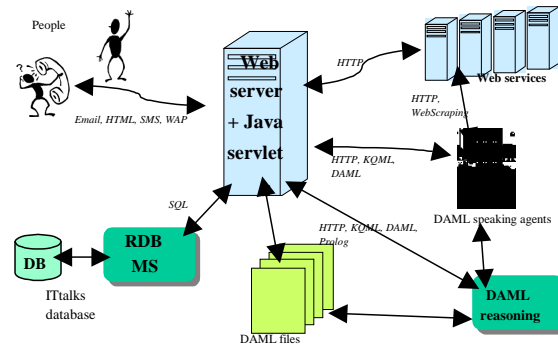
Fig. 4. The architecture for ITTALKS is built around a web server backed by a relational database. Interfaces are provided to human users, software agents and web services.
