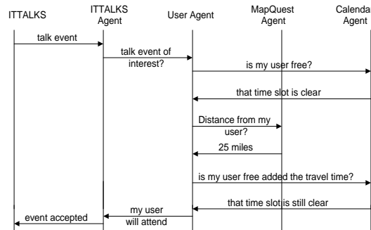
Fig. 6. Interactions between the various agents described in the ITTALKS/Agent scenario.
