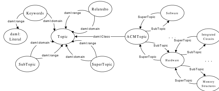
Fig. 7. The Ontologies used by ITTALKS are relatively simple, such as the topics ontology used to describe talk topics and user interests.
