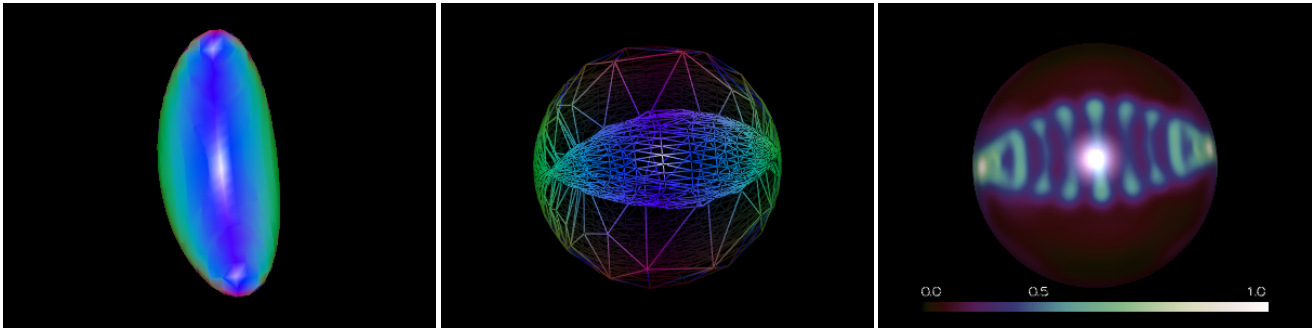
Figure 2: The model-view (left) and two different Gauss-views (center – mesh view and the splatted Gauss map – right) of an implicitly created shape. This viewpoint is a frontal perspective of the saddle-shaped section of a simple bean shape. The highlight on the fold of the meshed Gauss map indicates that there are three separate locations on the model that share the same normal, showing three highlights (left).
