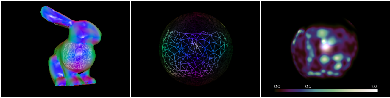
Figure 4: An example of brushing a complex model. When a patch of polygons in the model-view (left) is selected, the corresponding patch is highlighted in the Gauss maps (center and right). This technique helps disambiguate areas, focusing the visualization or regions of interest.
