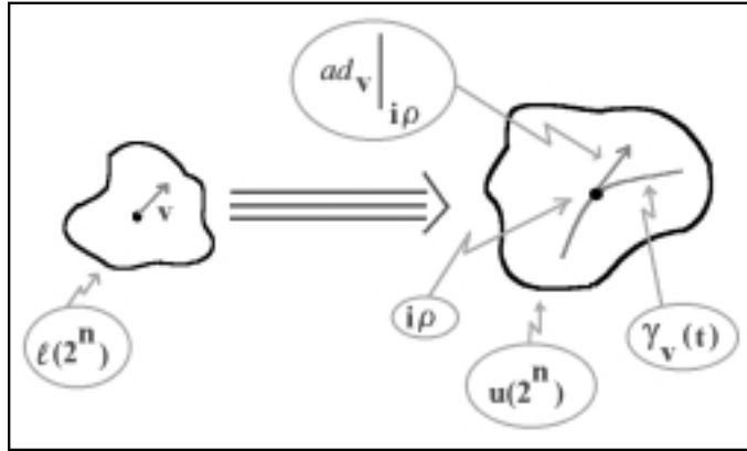
Figure 3. Induced infinitesimal action
