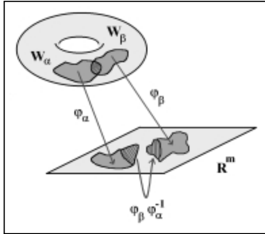
Figure 7. An atlas is smooth if every \varphi_\beta \varphi_\alpha^{-1} is smooth when defined.
