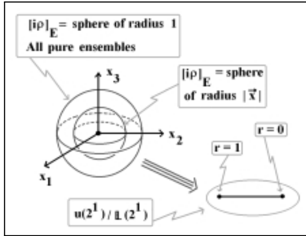
Figure 5. The Bloch “sphere”
