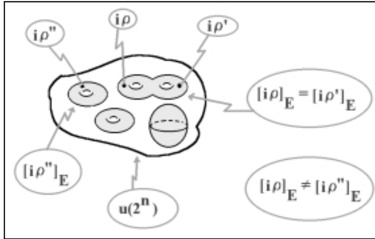
Figure 2. Quantum entanglement classes.
