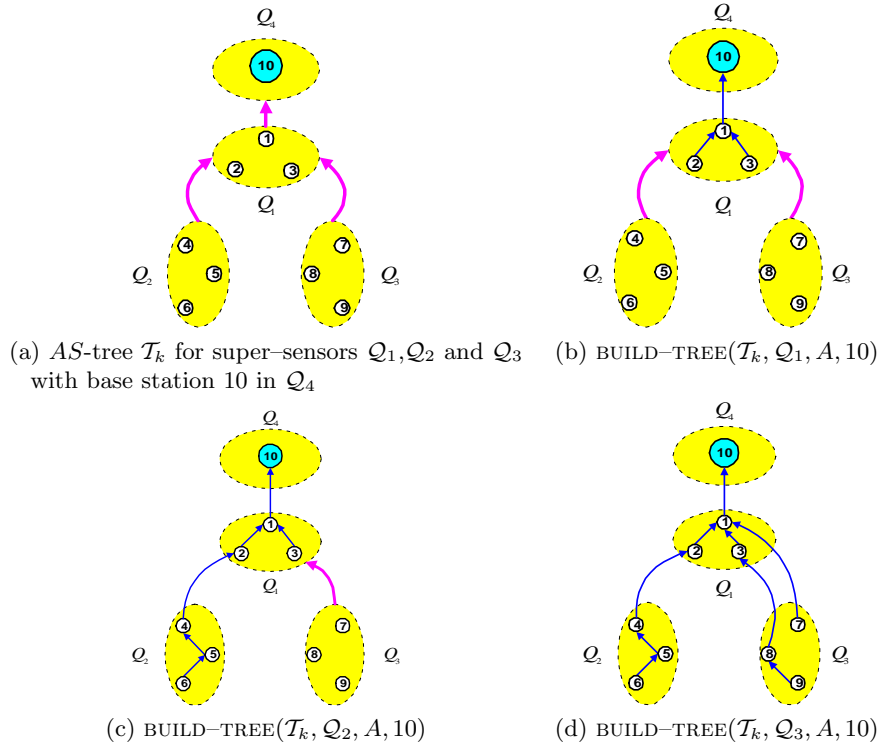
Figure 5: Illustration of the BUILD-TREE procedure for an AS-tree \mathcal{T}_k . Sensors 1, 2, \dots , 9 are partitioned among super-sensors \mathcal{Q}_1 , \mathcal{Q}_2 , and \mathcal{Q}_3 . Super-sensor \mathcal{Q}_4 contains the base station 10. The aggregation tree A is used for collecting one data packet from each sensor and transmitting to the base station.
