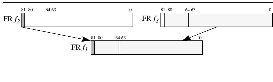
Figure 6-8. Floating-point Merge Sign Operation
