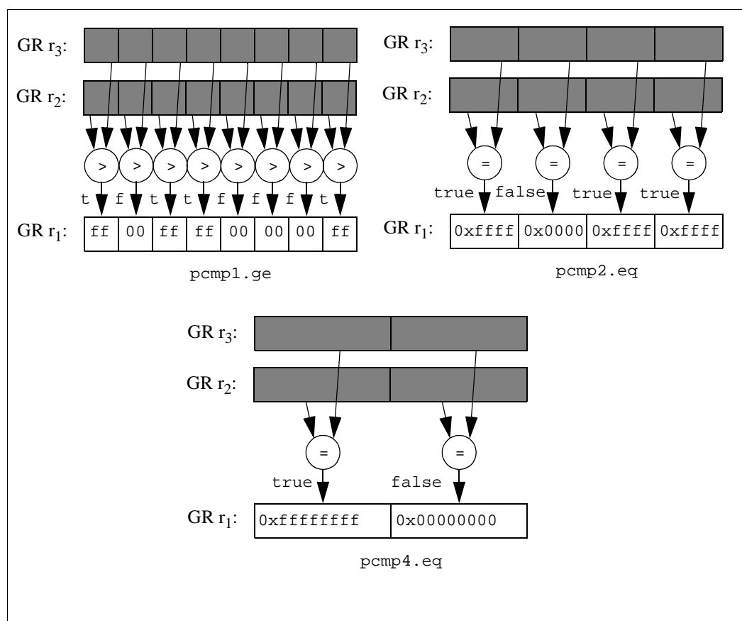
Figure 6-31. Parallel Compare Example
