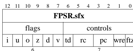
Figure 5-3. Floating-point Status Field Format
