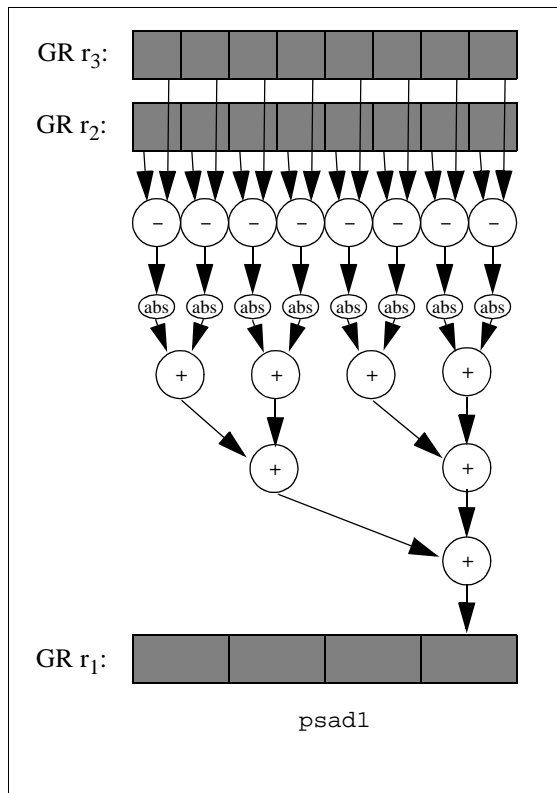
Figure 6-36. Parallel Sum of Absolute Difference Example
