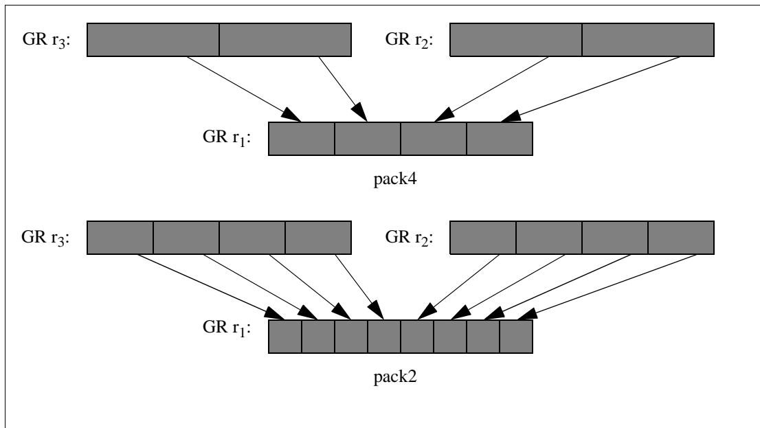
Figure 6-26. Pack Operation
