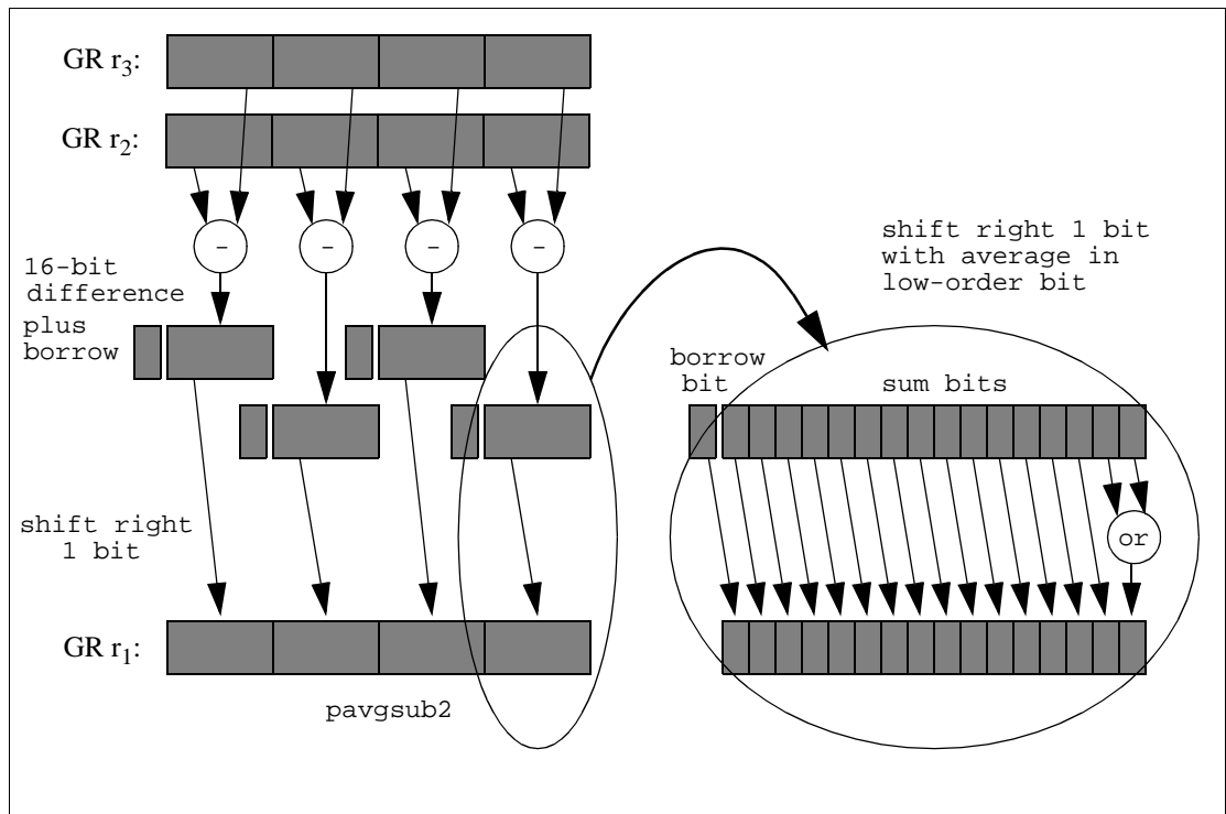
Figure 6-30. Parallel Average Subtract Example
