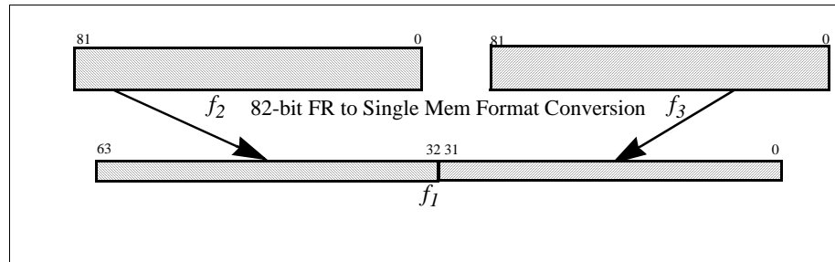
Figure 6-13. Floating-point Pack
