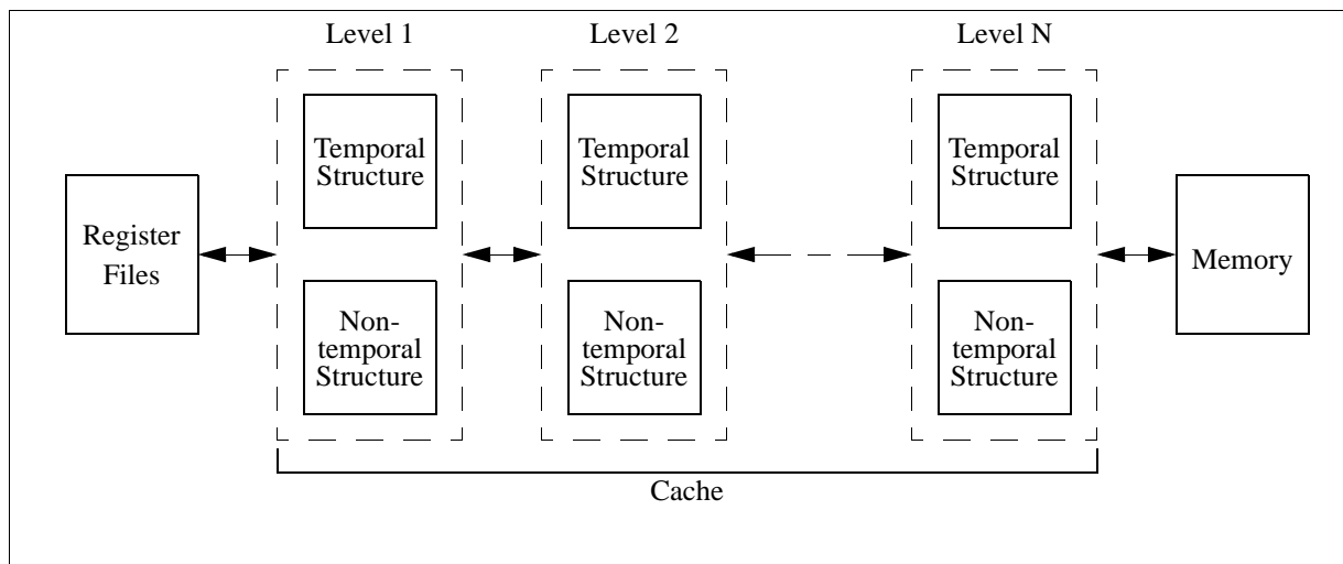
Figure 4-4. Memory Hierarchy
