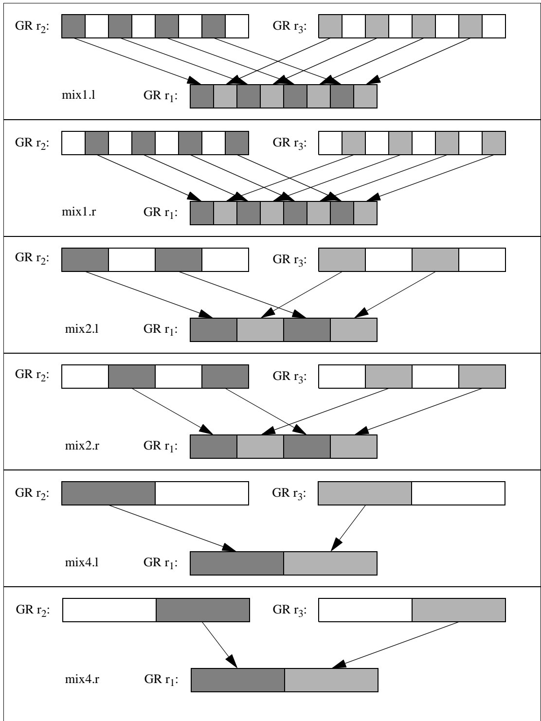
Figure 6-23. Mix Example
