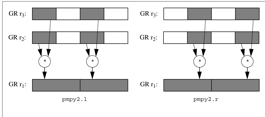
Figure 6-34. Parallel Multiply Operation
