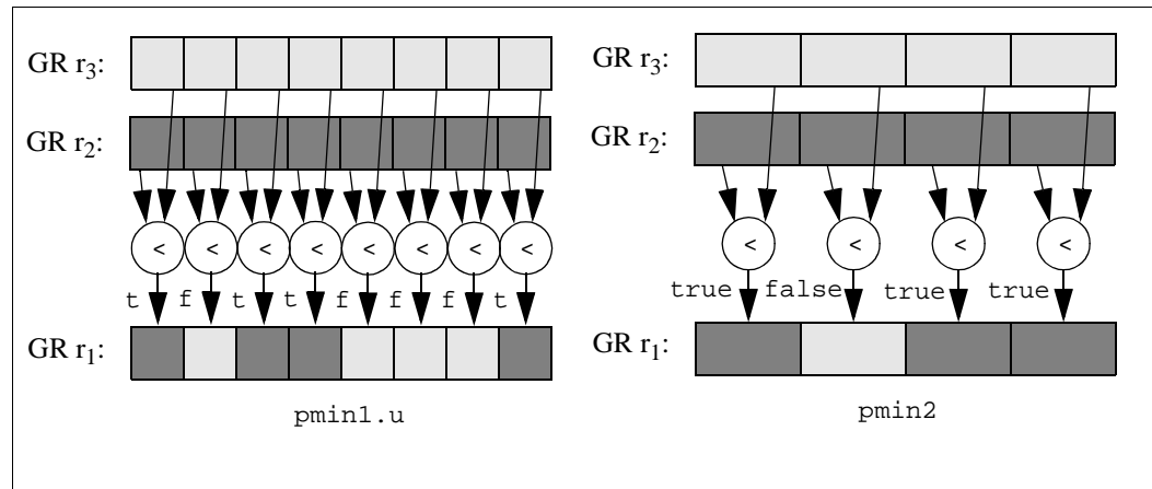
Figure 6-33. Parallel Minimum Example
