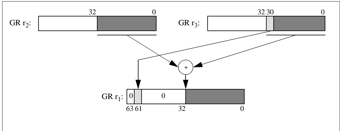
Figure 6-1. Add Pointer
