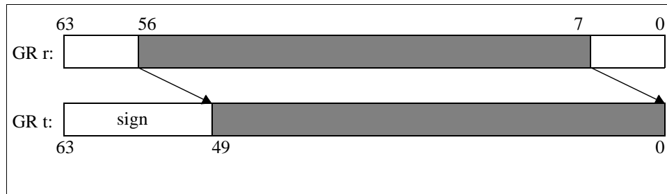
Figure 6-6. Extract Example
