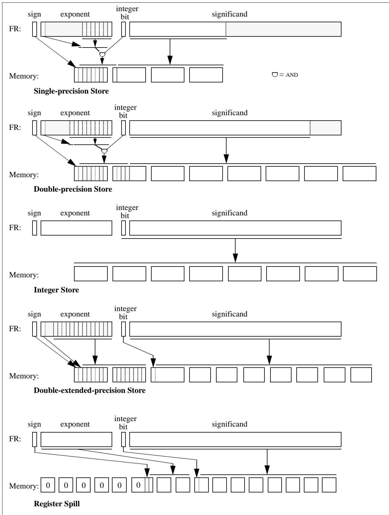
Figure 5-7. Floating-point Register to Memory Data Translation
