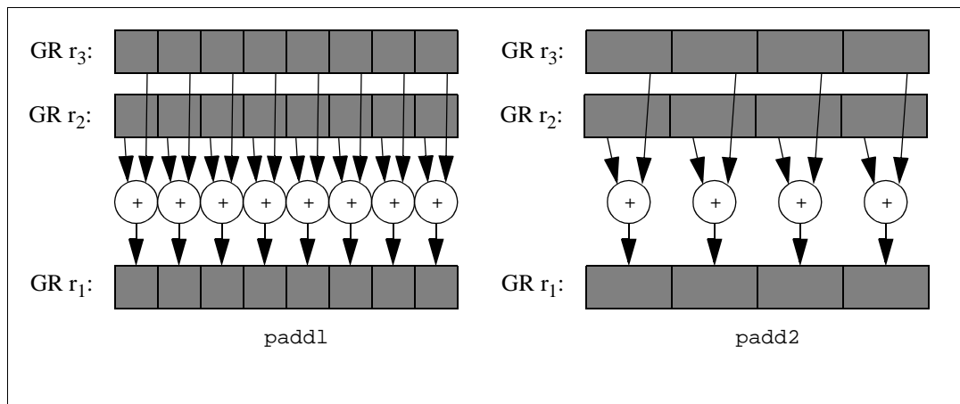
Figure 6-27. Parallel Add Examples
