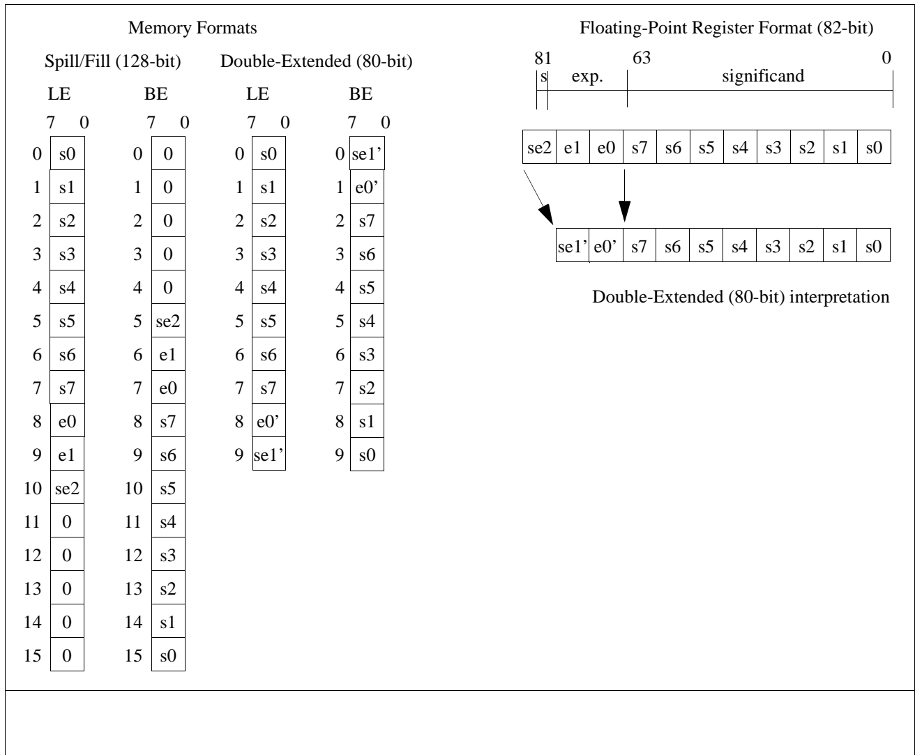
Figure 5-8. Spill/Fill and Double-Extended (80-bit) Floating-point Memory Formats
