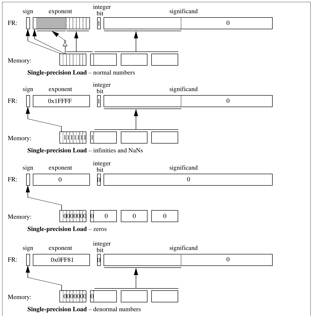
Figure 5-4. Memory to Floating-point Register Data Translation – Single Precision
