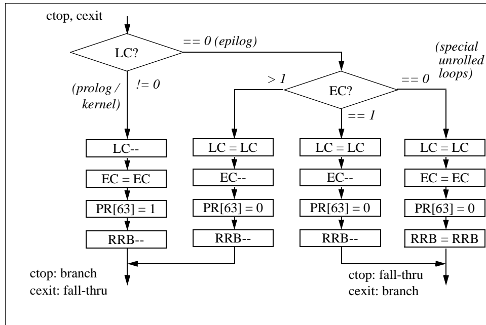
Figure 6-3. Operation of br.ctop and br.cexit
