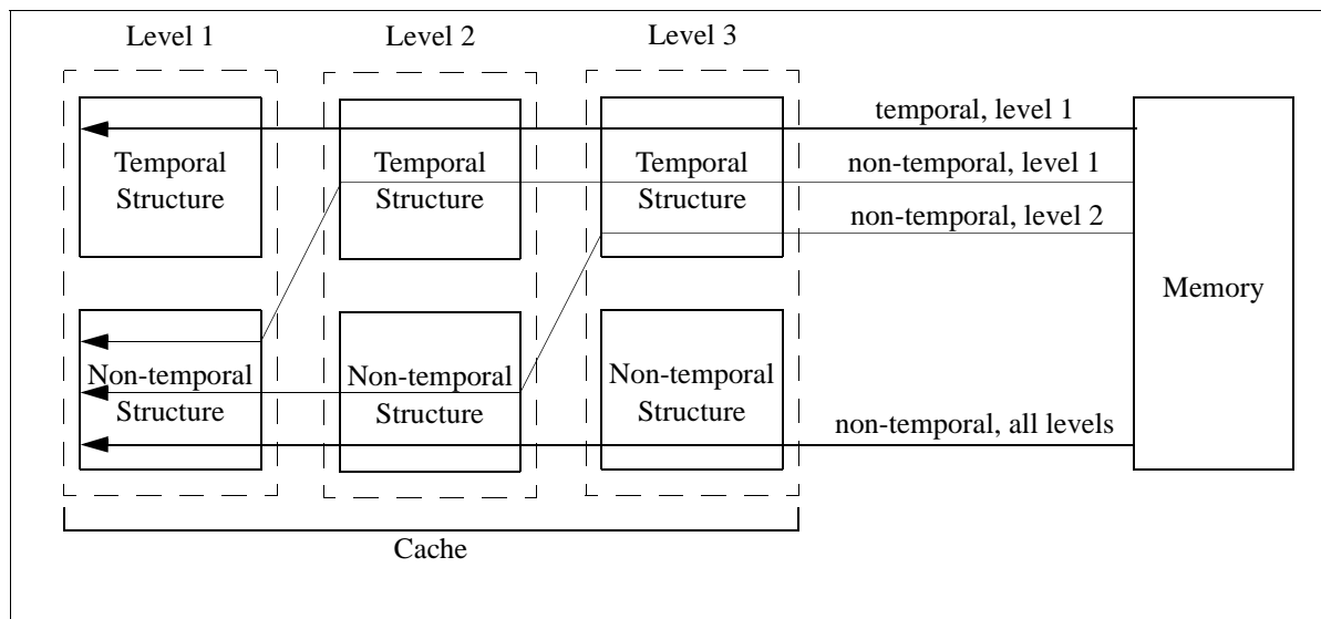
Figure 4-5. Allocation Paths Supported in the Memory Hierarchy
