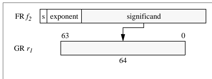
Figure 6-22. Function of getf.sig
