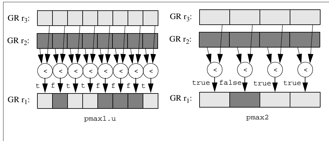
Figure 6-32. Parallel Maximum Example
