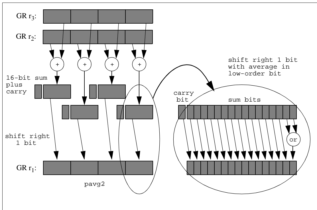
Figure 6-28. Parallel Average Example
