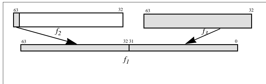
Figure 6-19. Floating-point Sign Extend Left
