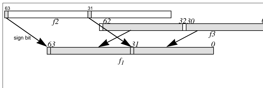
Figure 6-15. Floating-point Merge Sign Operation
