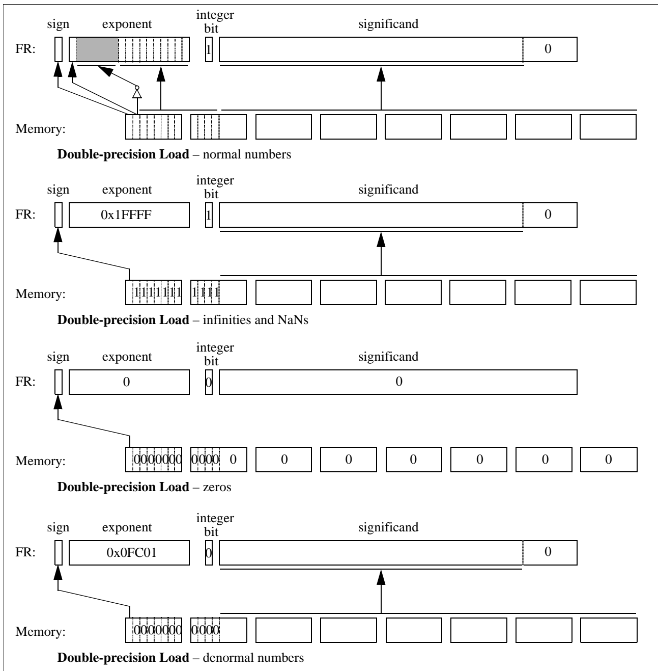
Figure 5-5. Memory to Floating-point Register Data Translation – Double Precision
