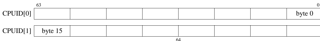
Figure 3-10. CPUID Registers 0 and 1 – Vendor Information
