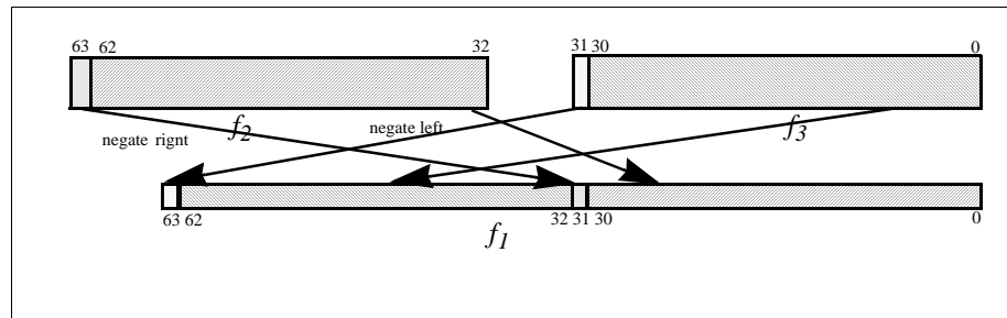
Figure 6-18. Floating-point Swap Negate Left or Right
