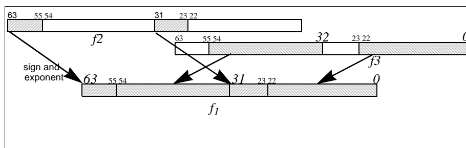
Figure 6-16. Floating-point Merge Sign and Exponent Operation
