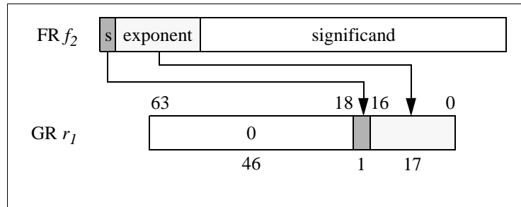
Figure 6-21. Function of getf.exp
