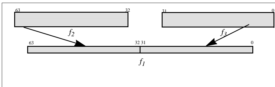
Figure 6-12. Floating-point Mix Left-Right
