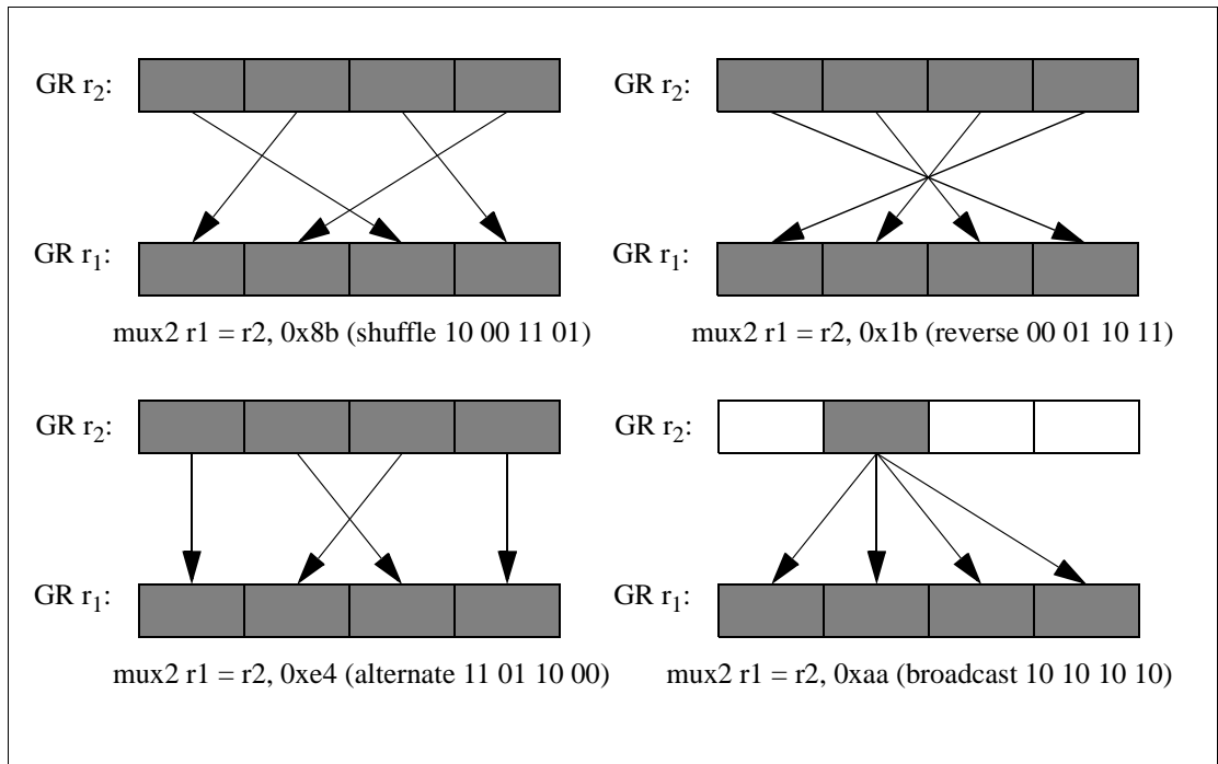
Figure 6-25. Mux2 Examples (16-bit elements)
