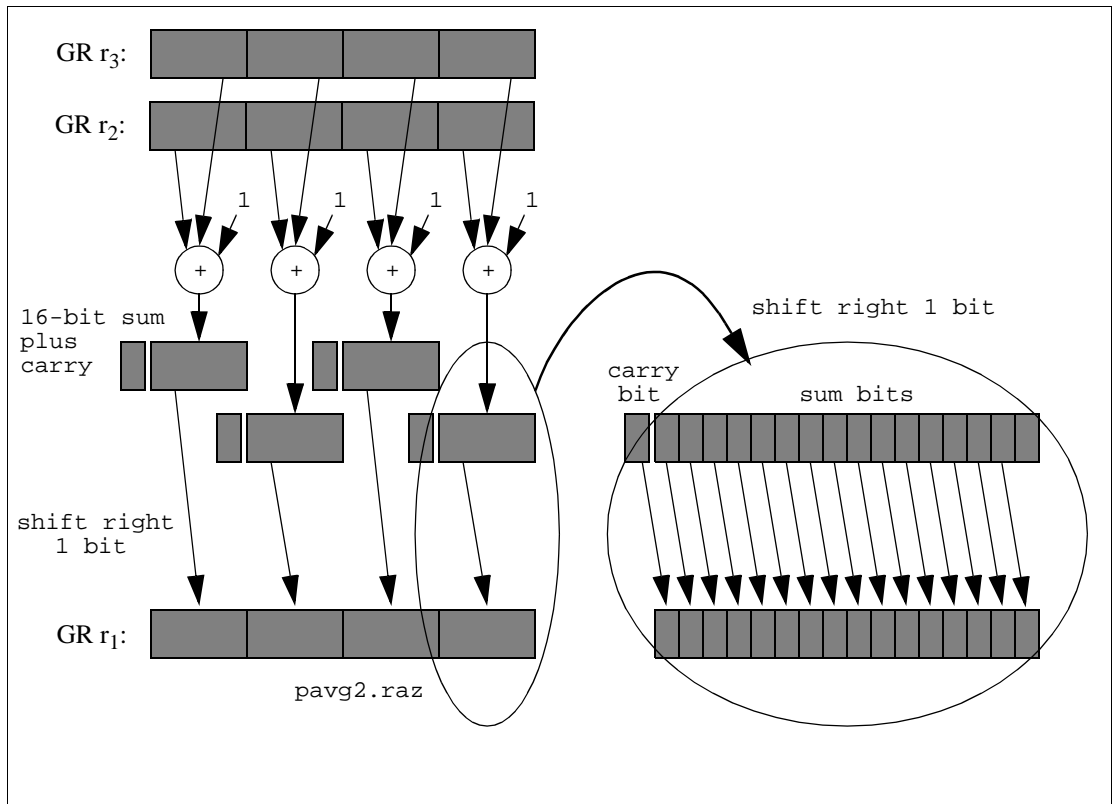
Figure 6-29. Parallel Average with Round Away from Zero Example
