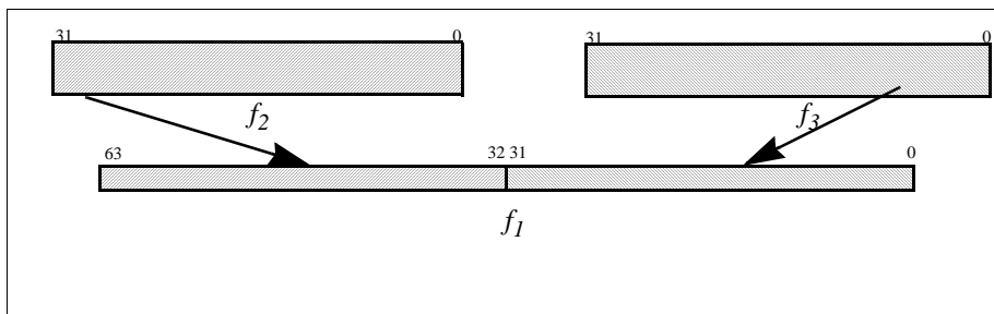
Figure 6-11. Floating-point Mix Right
