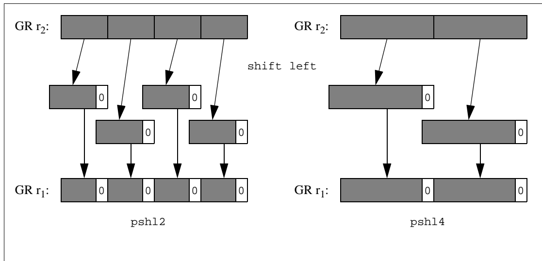
Figure 6-37. Parallel Shift Left Example
