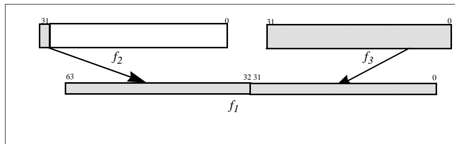
Figure 6-20. Floating-point Sign Extend Right
