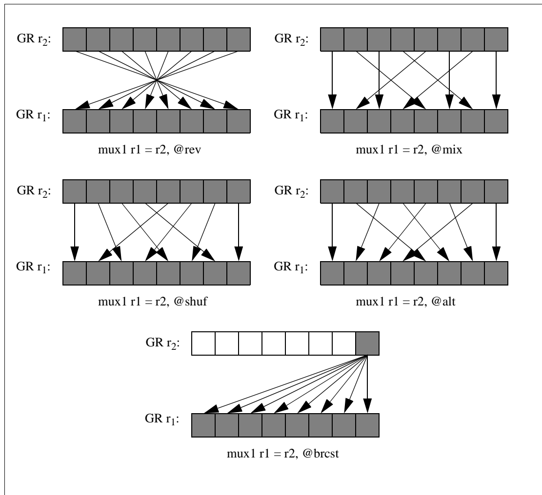
Figure 6-24. Mux1 Operation (8-bit elements)
