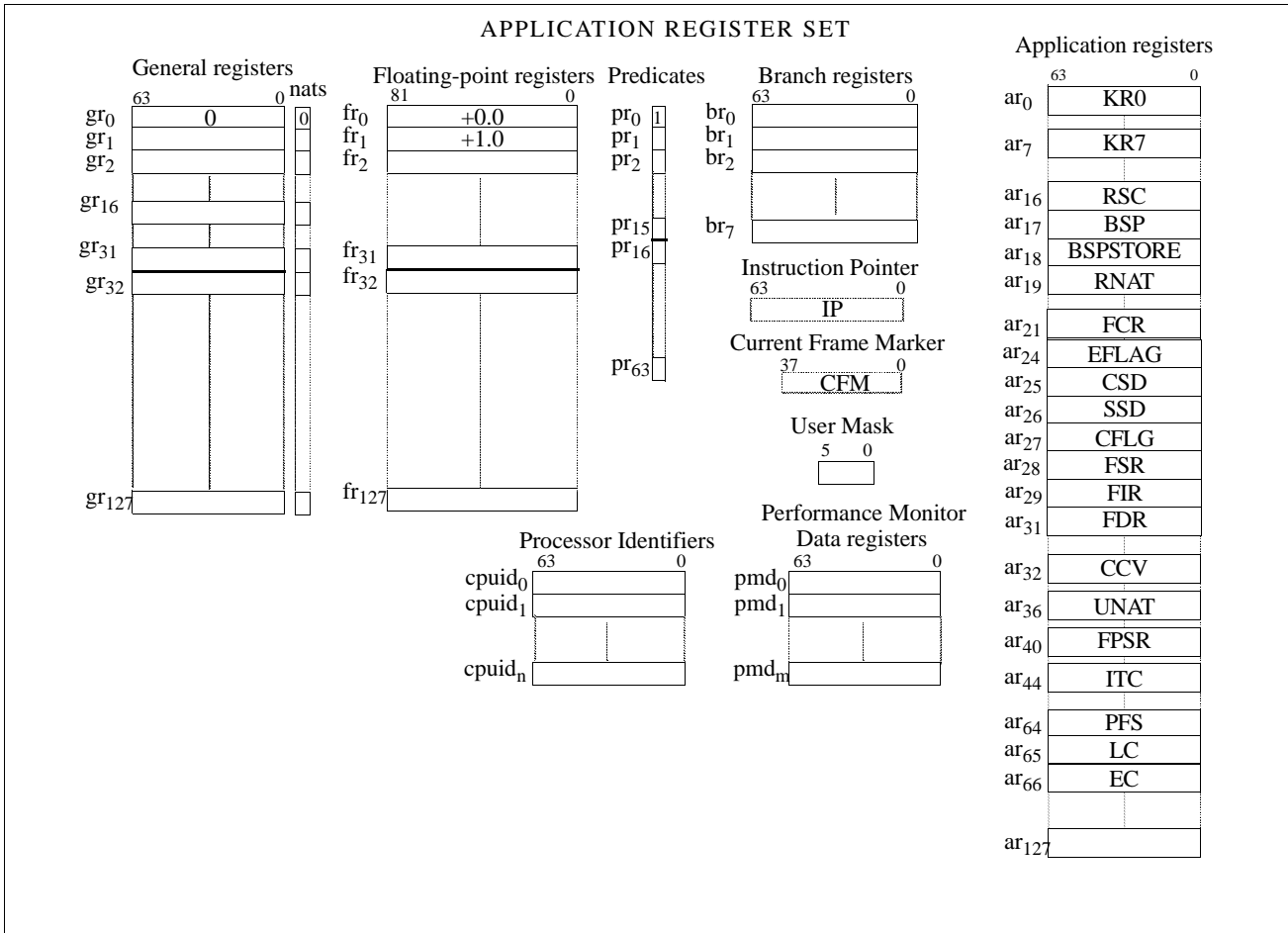
Figure 3-1. Application Register Model
