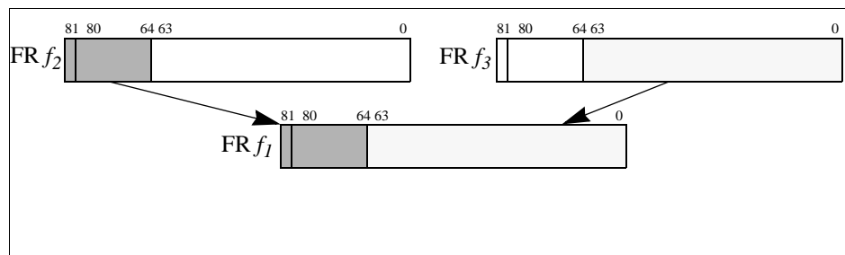
Figure 6-9. Floating-point Merge Sign and Exponent Operation
