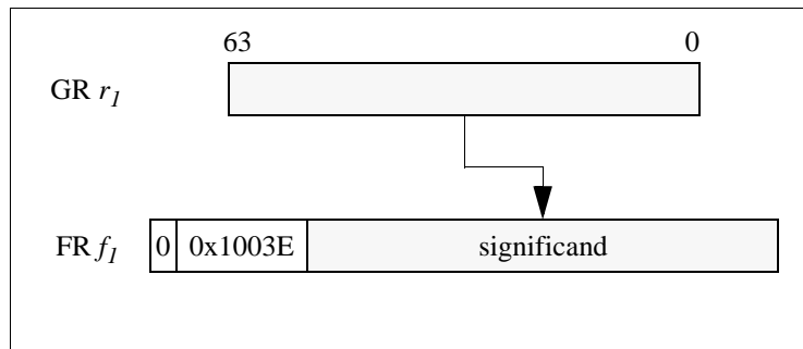
Figure 6-40. Function of setf.sig
