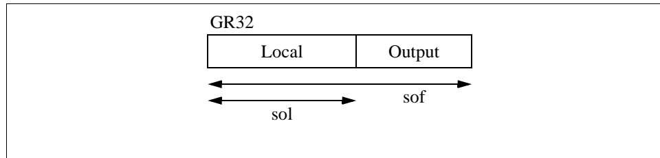
Figure 6-2. Stack Frame
