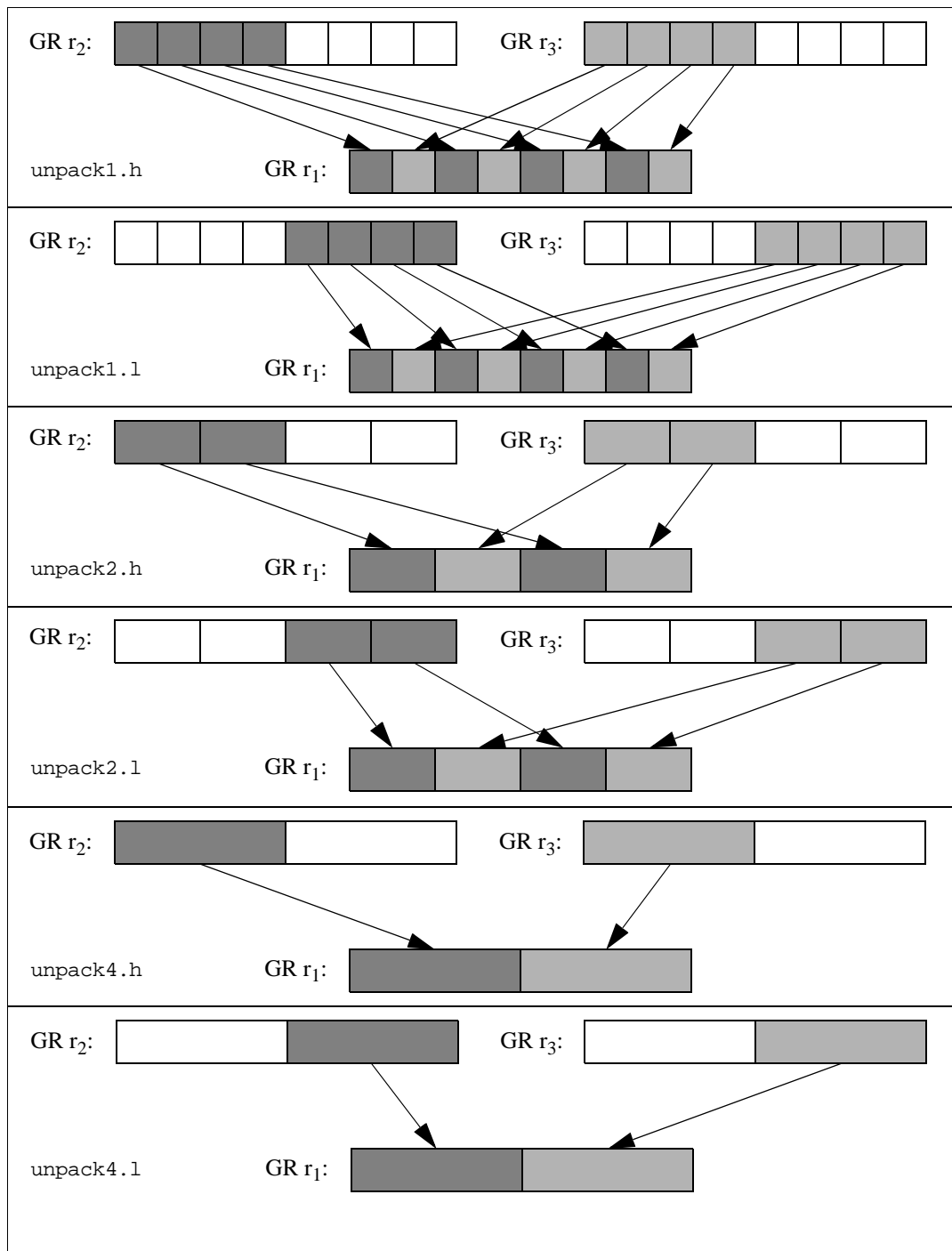
Figure 6-43. Unpack Operation
