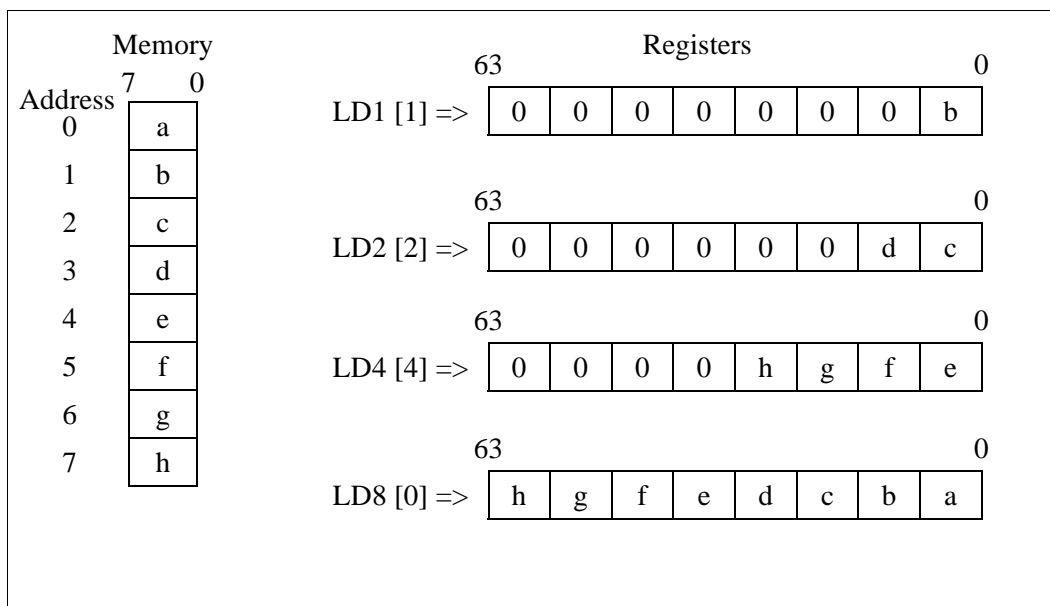
Figure 3-14. Little-endian Loads
