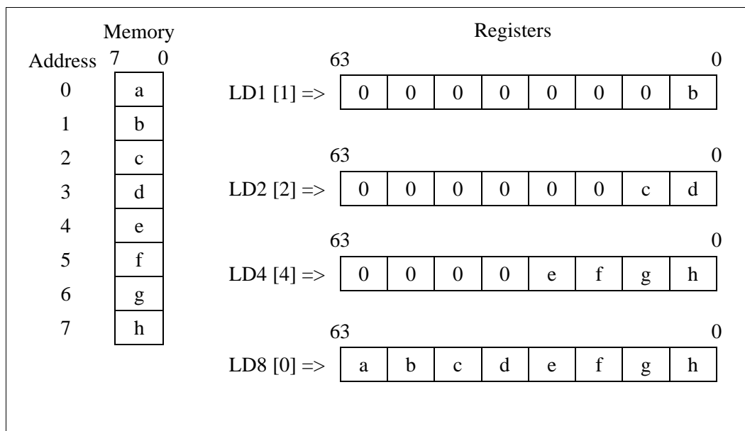
Figure 3-15. Big-endian Loads
