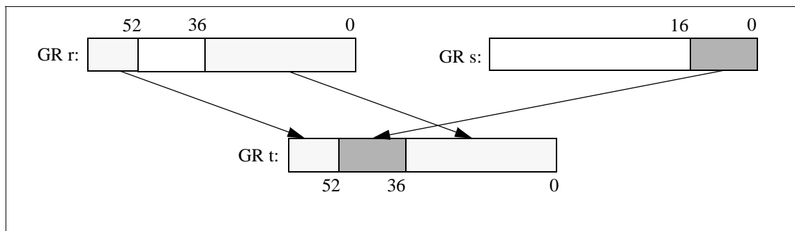
Figure 6-5. Deposit Example
