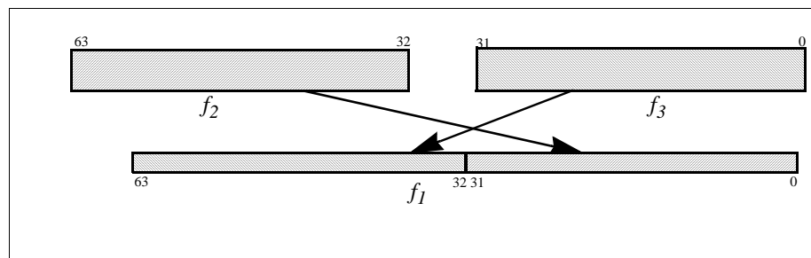
Figure 6-17. Floating-point Swap
