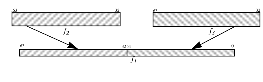
Figure 6-10. Floating-point Mix Left
