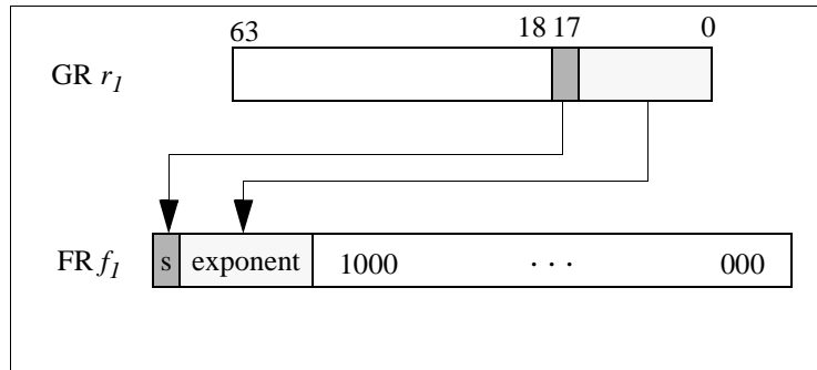
Figure 6-39. Function of setf.exp
