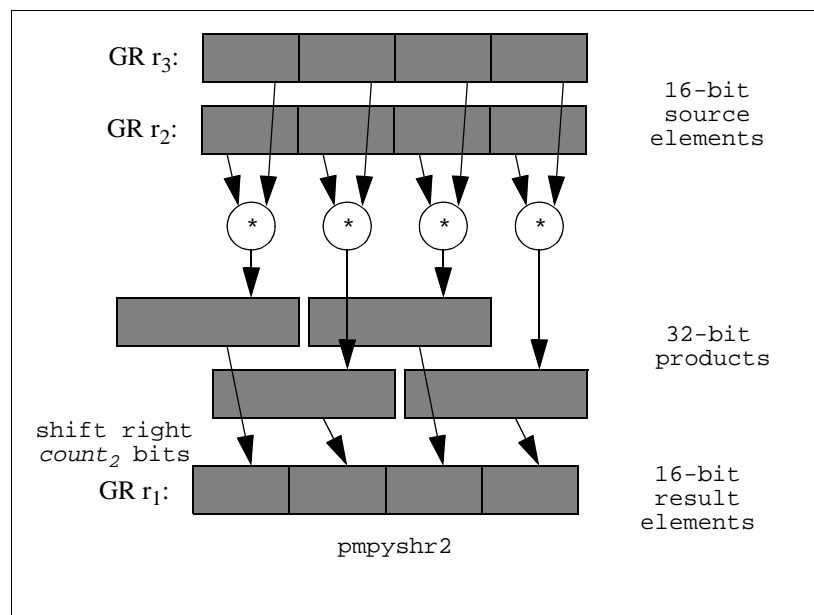
Figure 6-35. Parallel Multiply and Shift Right Operation
