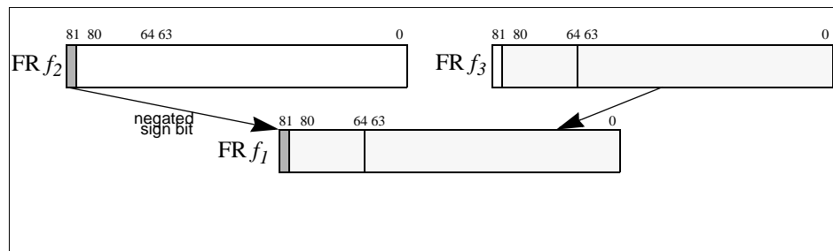
Figure 6-7. Floating-point Merge Negative Sign Operation
