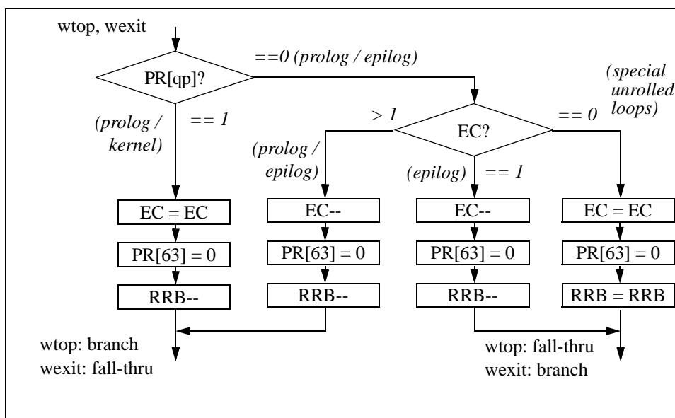
Figure 6-4. Operation of br.wtop and br.wexit
