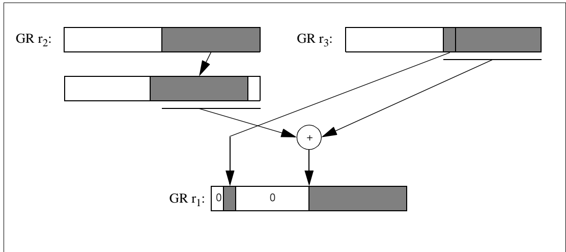
Figure 6-41. Shift Left and Add Pointer
