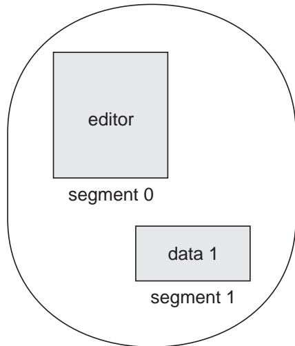
logical memory process P_1
