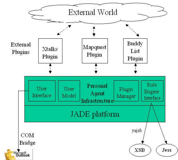
Figure 4: Personal Agent Architecture
